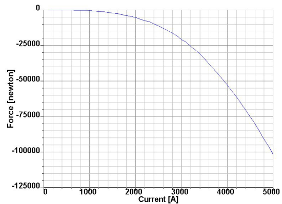
Figure 3.61: Residual axial force as a function of current during normal power cycling. The force will increase steadily and will never change direction.
