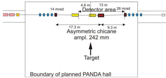
Figure 2.15: Detail of the HESR layout showing the straight section where the \bar{P} ANDA experiment is located. The \bar{P} ANDA detectors will be within the “Detector area”. The \bar{P} ANDA solenoid and compensating solenoid (to the left of it) are indicated in yellow, the \bar{P} ANDA dipole and the 2 dipoles of the chicane in red, and the quadrupoles in blue.
