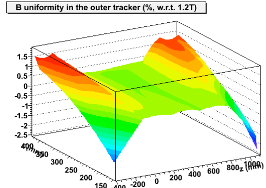
Figure 3.63: \Delta B/B distribution over the outer tracker region at 60% of the nominal current.
