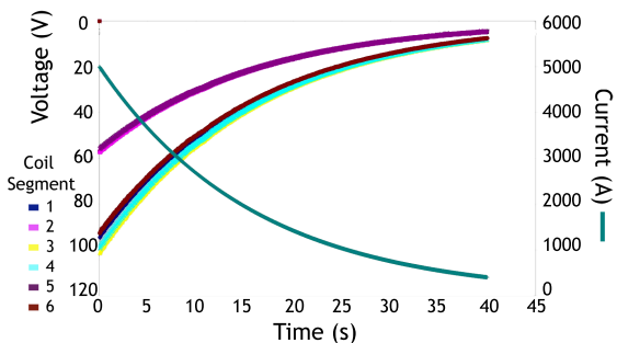
Figure 3.12: Voltage and current evolution in the coil after a quench as a function of time. The coil was divided into 6 sectors, the 3 sub-coils divided into the 2 layers. The calculation refers to the same scenario as 3.11 (courtesy AS-G Superconductors).
