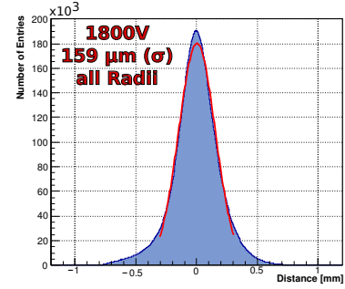
Figure 3: Residual distribution. The spatial resolution is defined as the sigma of a Gaussian fit and is around 160 \mu\text{m} .
