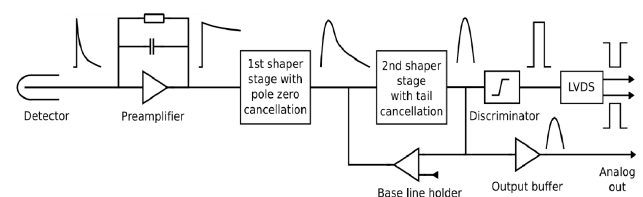
Figure 1: Block diagram of the PASTTREC chip.
