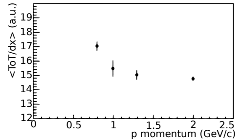
Figure 4: ToT/dx for different beam momenta.
