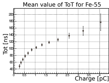
Figure 2: Time-over-threshold and charge correlation. Data taken with a Fe^{55} source. The correlation is used to translate the ToT to charge values.
